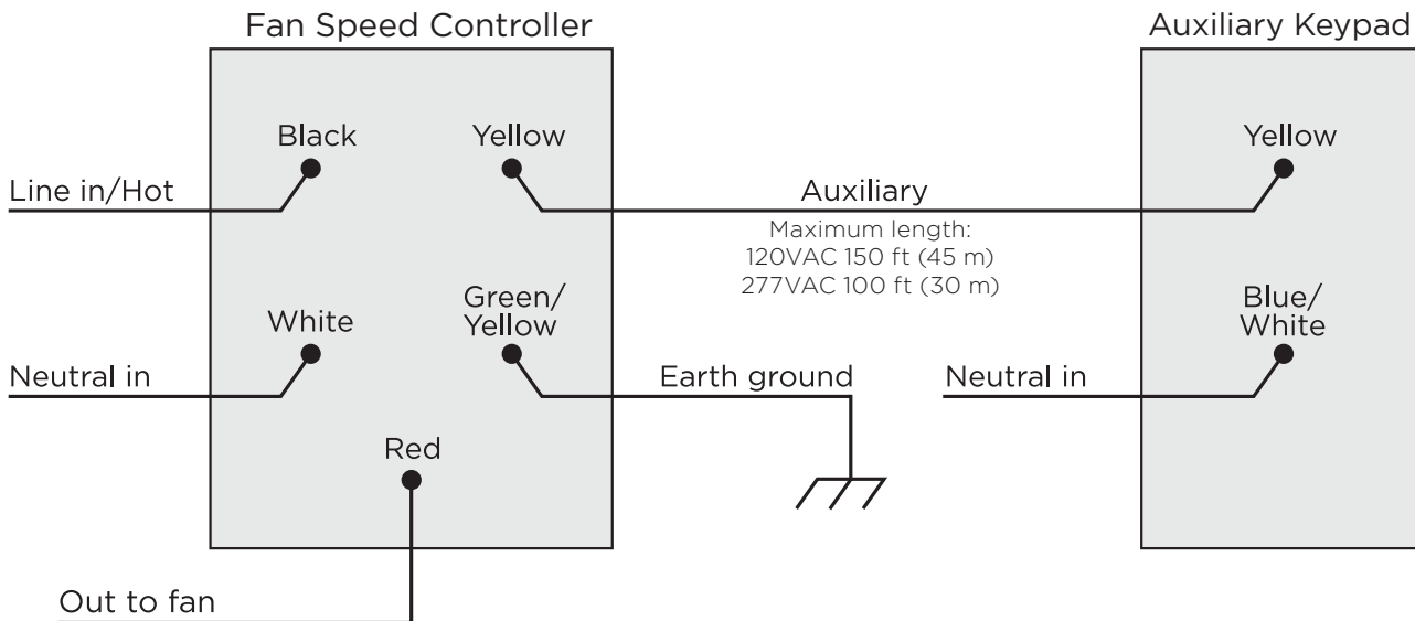
Figure 4. Multiple device location using Auxiliary Keypad
