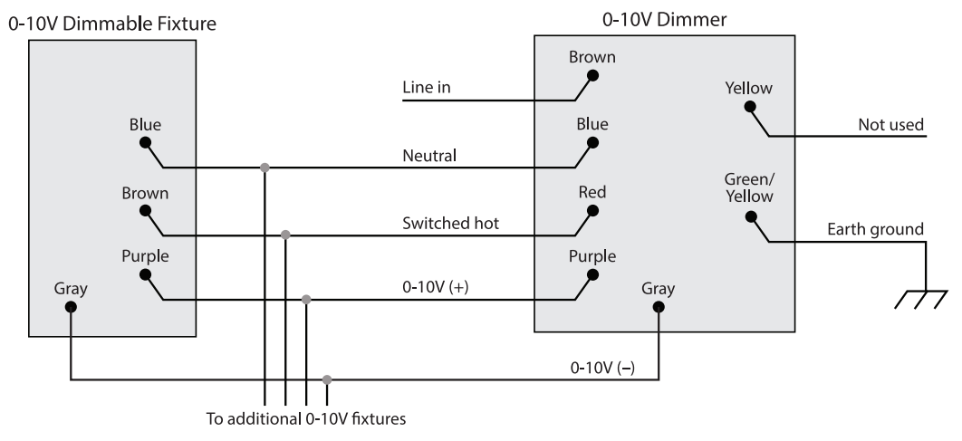
Figure 2. Single device location, with neutral connection
