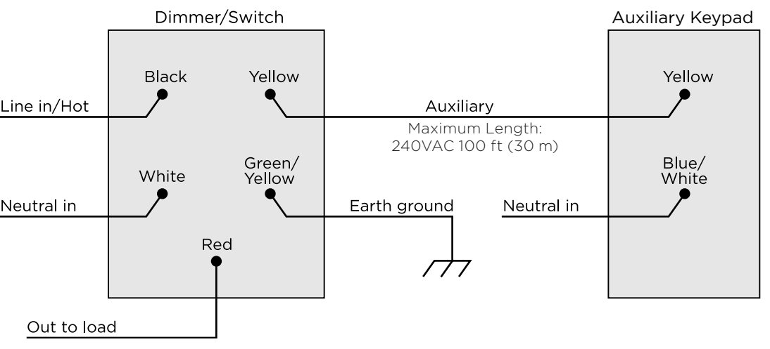
Figure 4. Multiple device location using Configurable Keypad, neutral required
