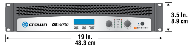
Figure 2.1 Dimensions
