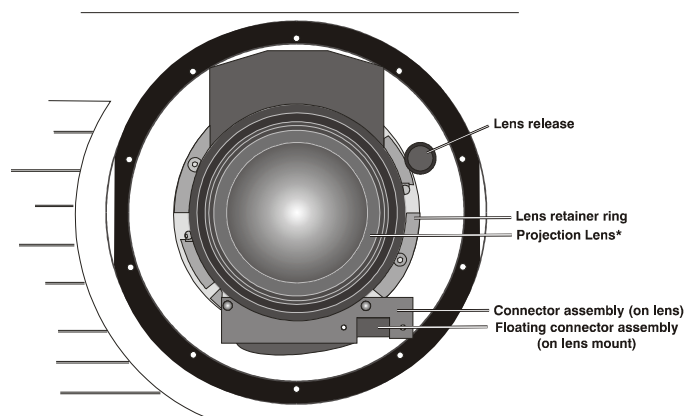
Figure 4-11 Lens Parts
