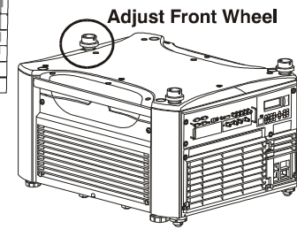
Figure 2-18 Adjust Front Wheel
