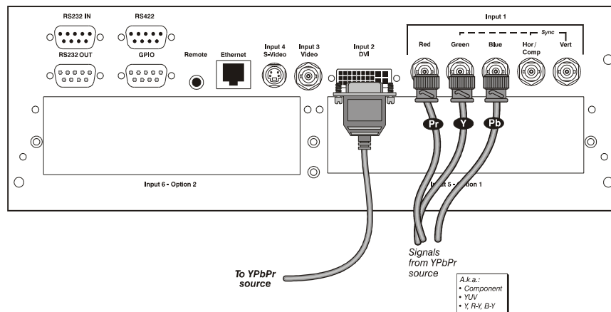
Figure 2-29 Connecting YPbPr
