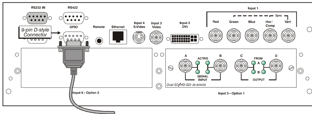
Figure 2-34 GPIO Port
