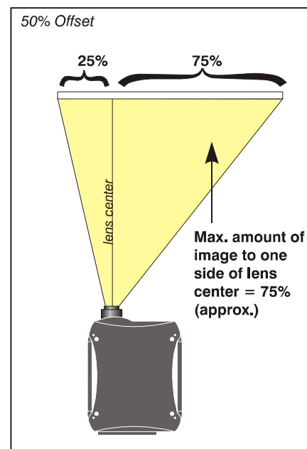
Figure 2-24 Maximum Horizontal Offset
