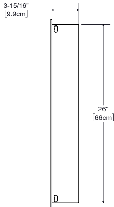
Right view
