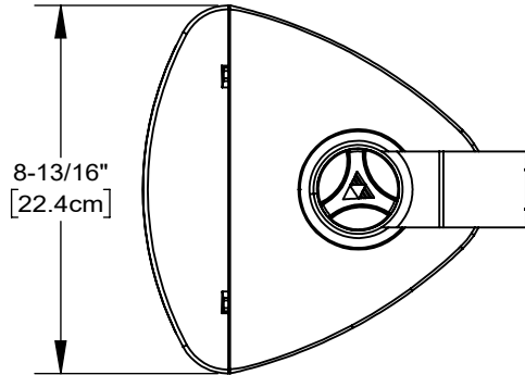
Right view
